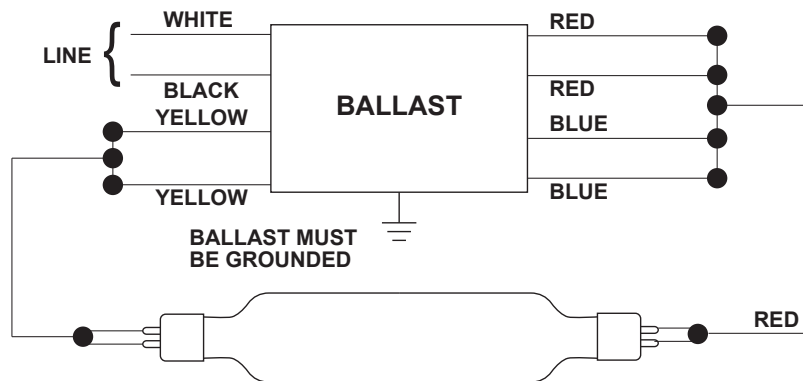
Wiring Diagram 1
